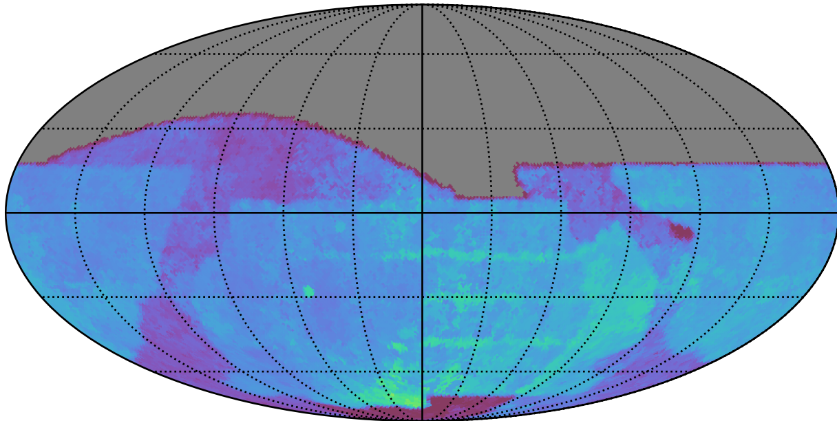
baseline_v2.0_10yrs All sky i band: 80thPercentile Season Length
