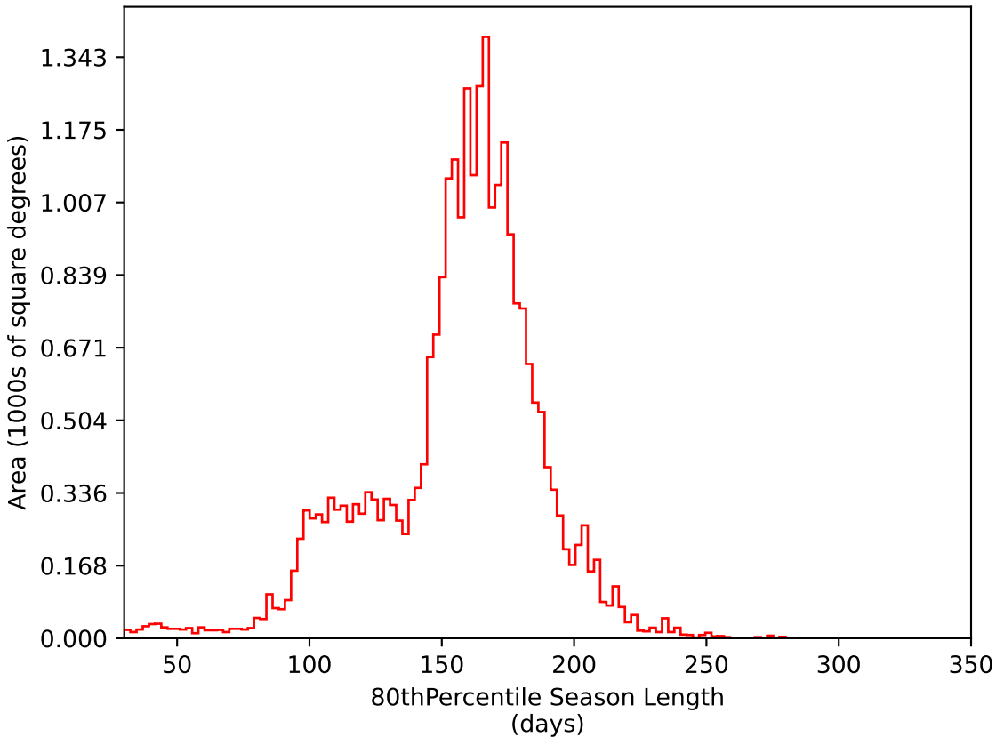
baseline_v2.0_10yrs All sky i band: 80thPercentile Season Length
