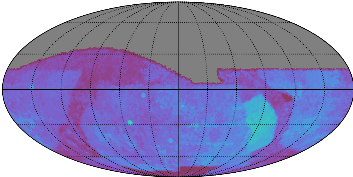
baseline_v2.0_10yrs All sky g band: 80thPercentile Season Length
