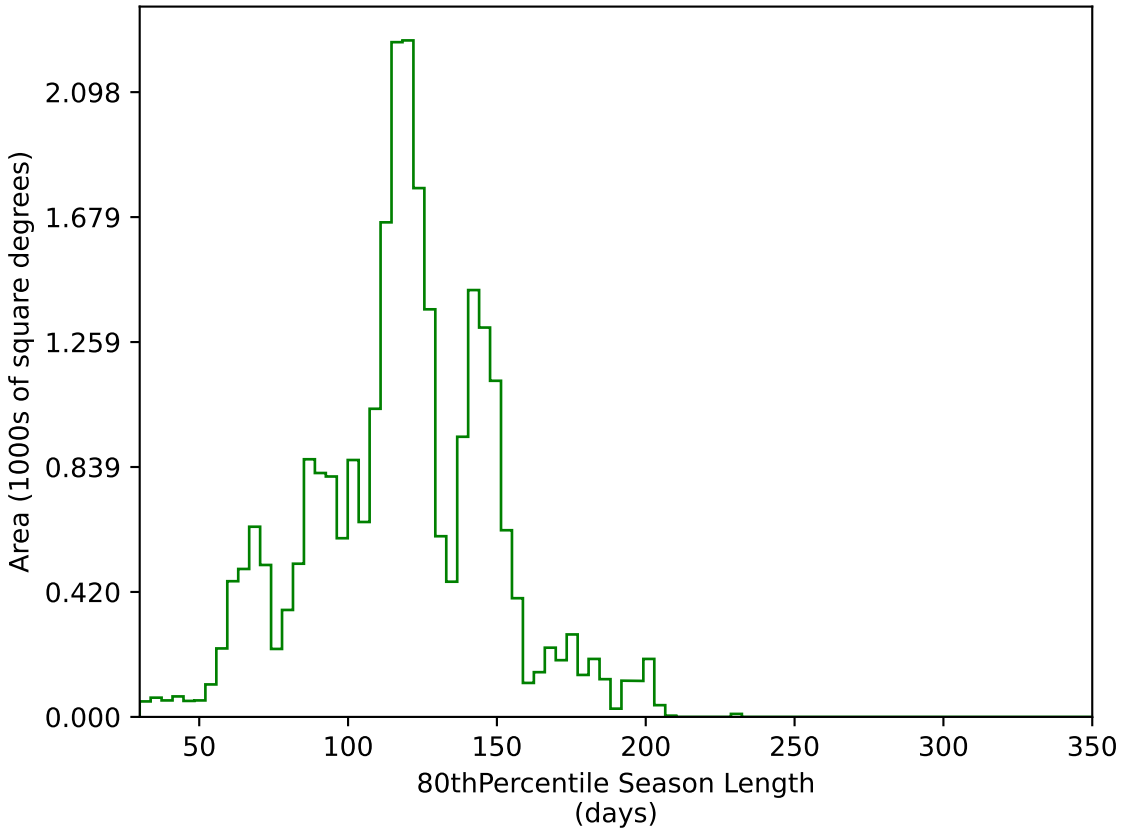
baseline_v2.0_10yrs All sky g band: 80thPercentile Season Length
