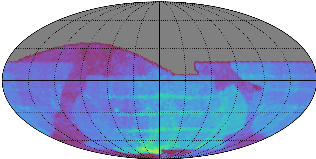
baseline_v2.0_10yrs All sky all bands: 80thPercentile Season Length
