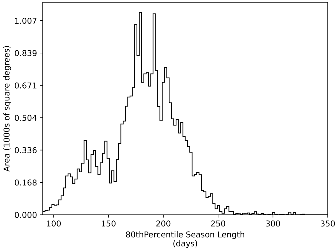
baseline_v2.0_10yrs All sky all bands: 80thPercentile Season Length
