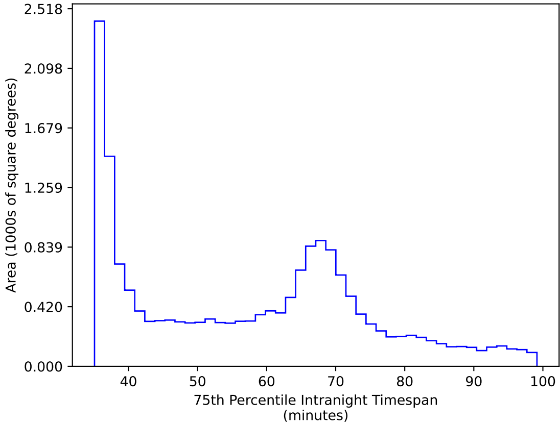
baseline_v2.0_10yrs WFD zy bands: 75th Percentile Intranight Timespan
