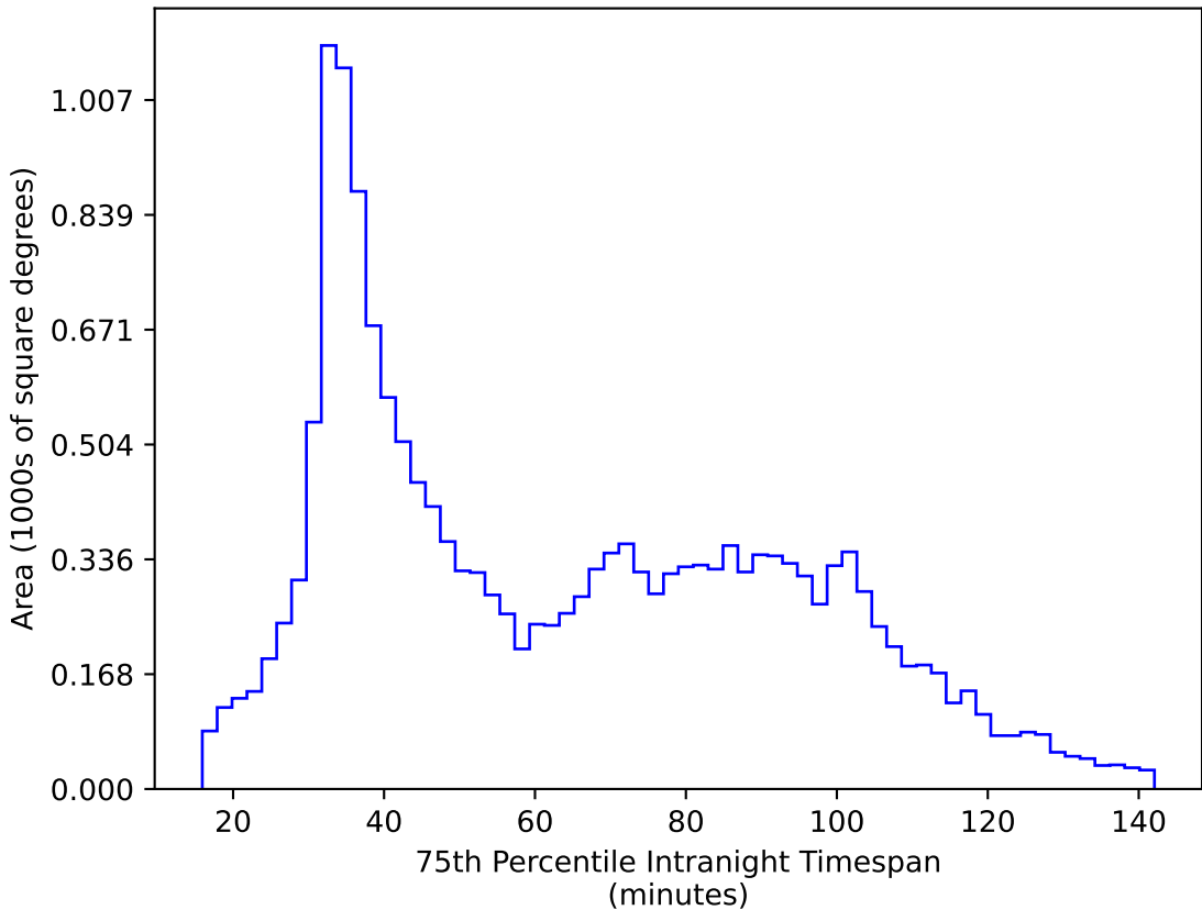
baseline_v2.0_10yrs WFD z band: 75th Percentile Intranight Timespan
