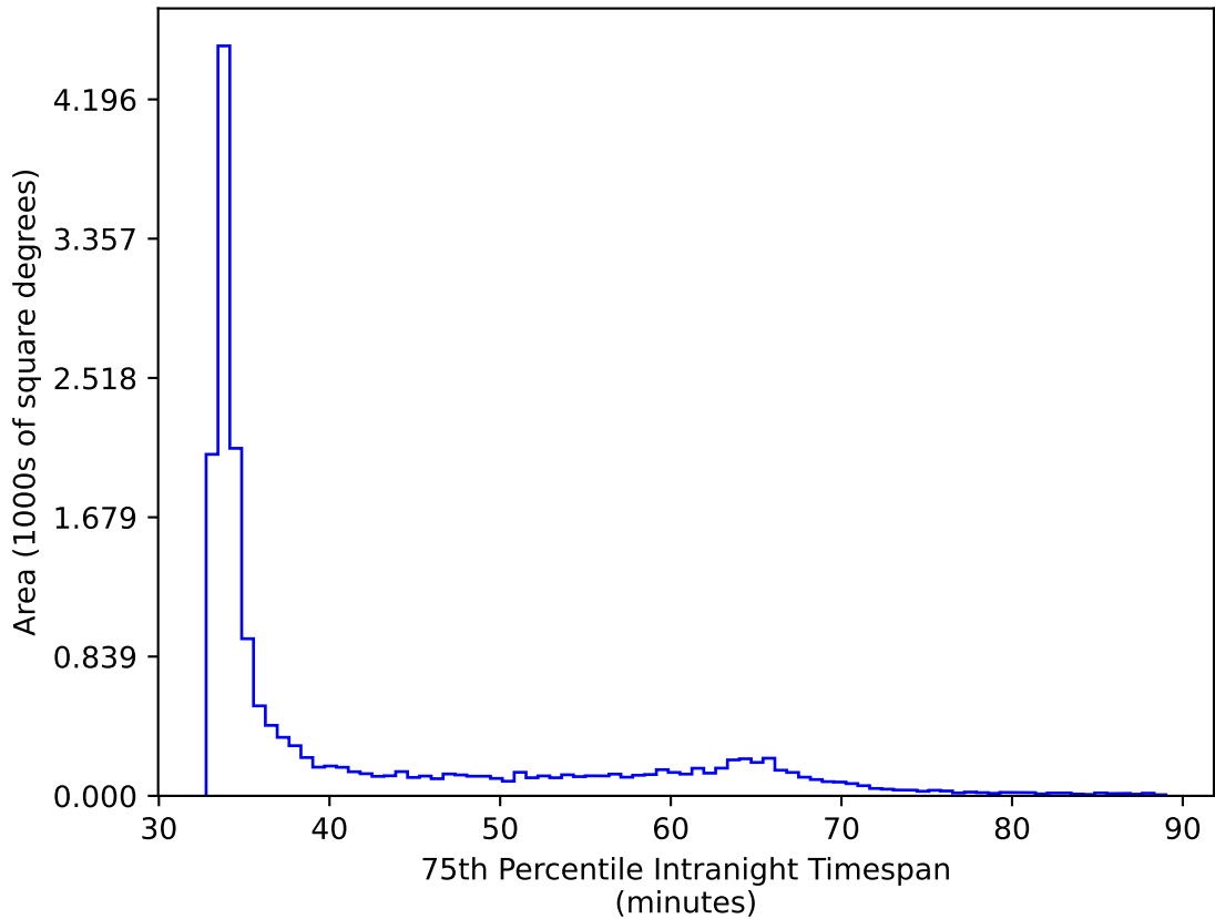
baseline_v2.0_10yrs WFD y band: 75th Percentile Intranight Timespan
