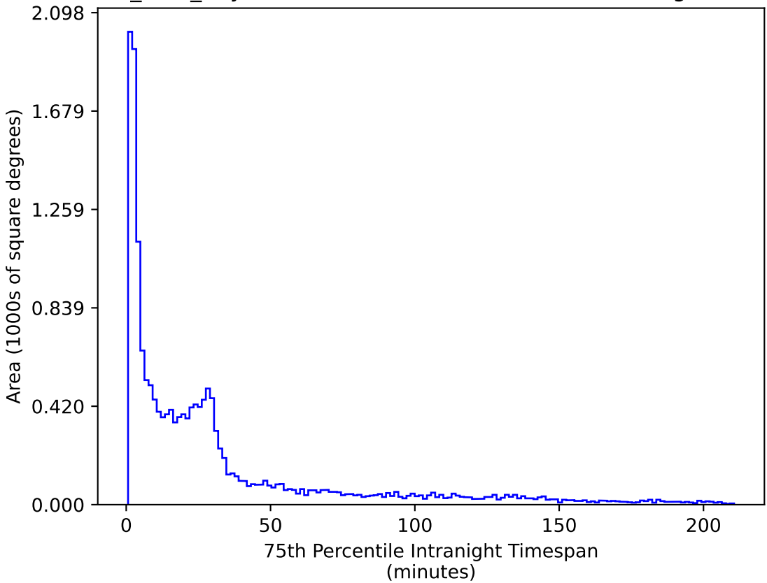
baseline_v2.0_10yrs WFD u band: 75th Percentile Intranight Timespan
