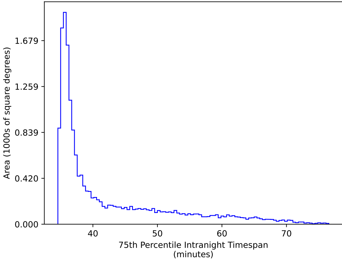
baseline_v2.0_10yrs WFD ri bands: 75th Percentile Intranight Timespan
