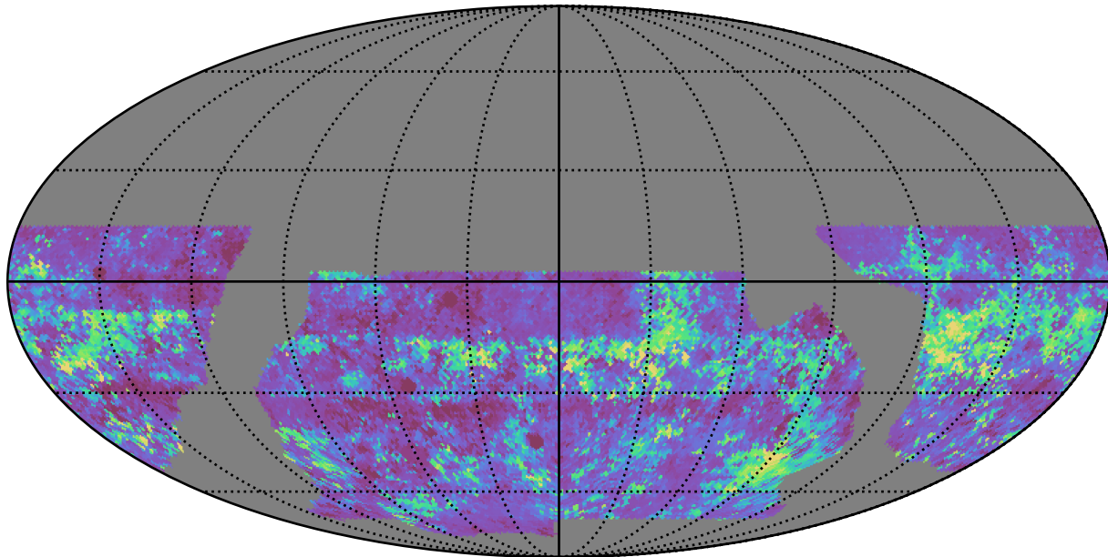
baseline_v2.0_10yrs WFD r band: 75th Percentile Intranight Timespan
