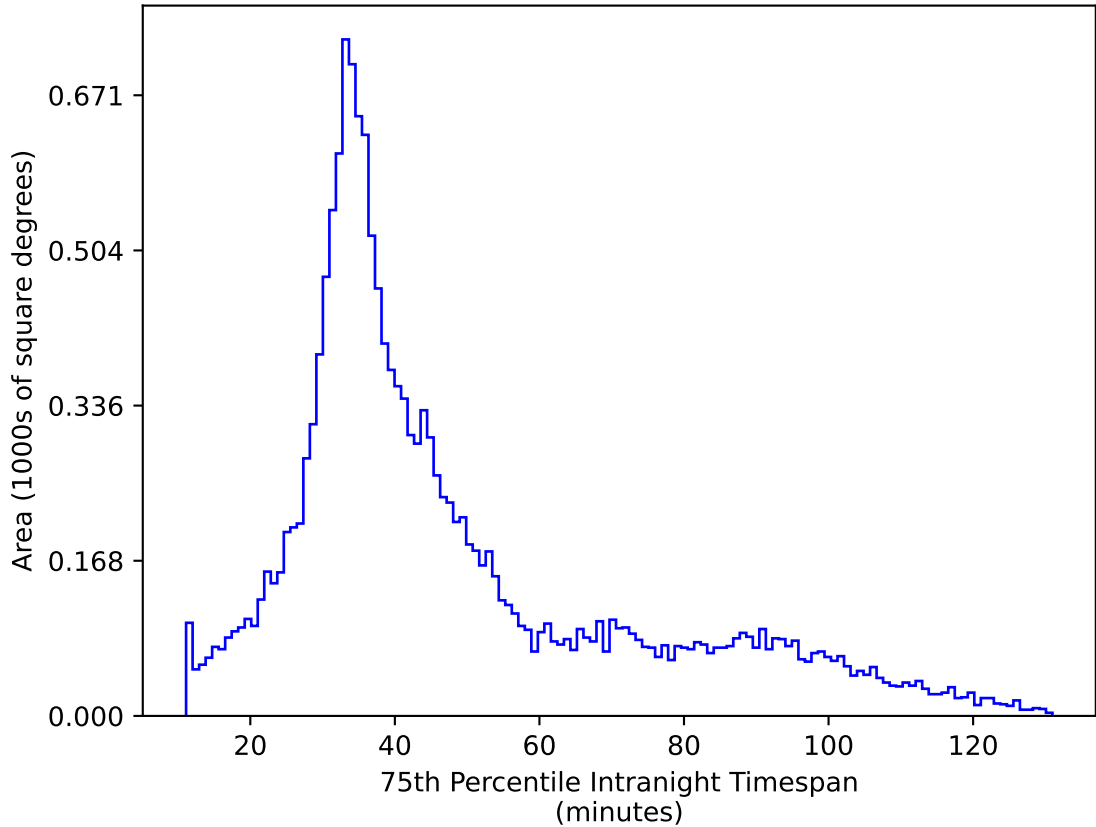
baseline_v2.0_10yrs WFD r band: 75th Percentile Intranight Timespan
