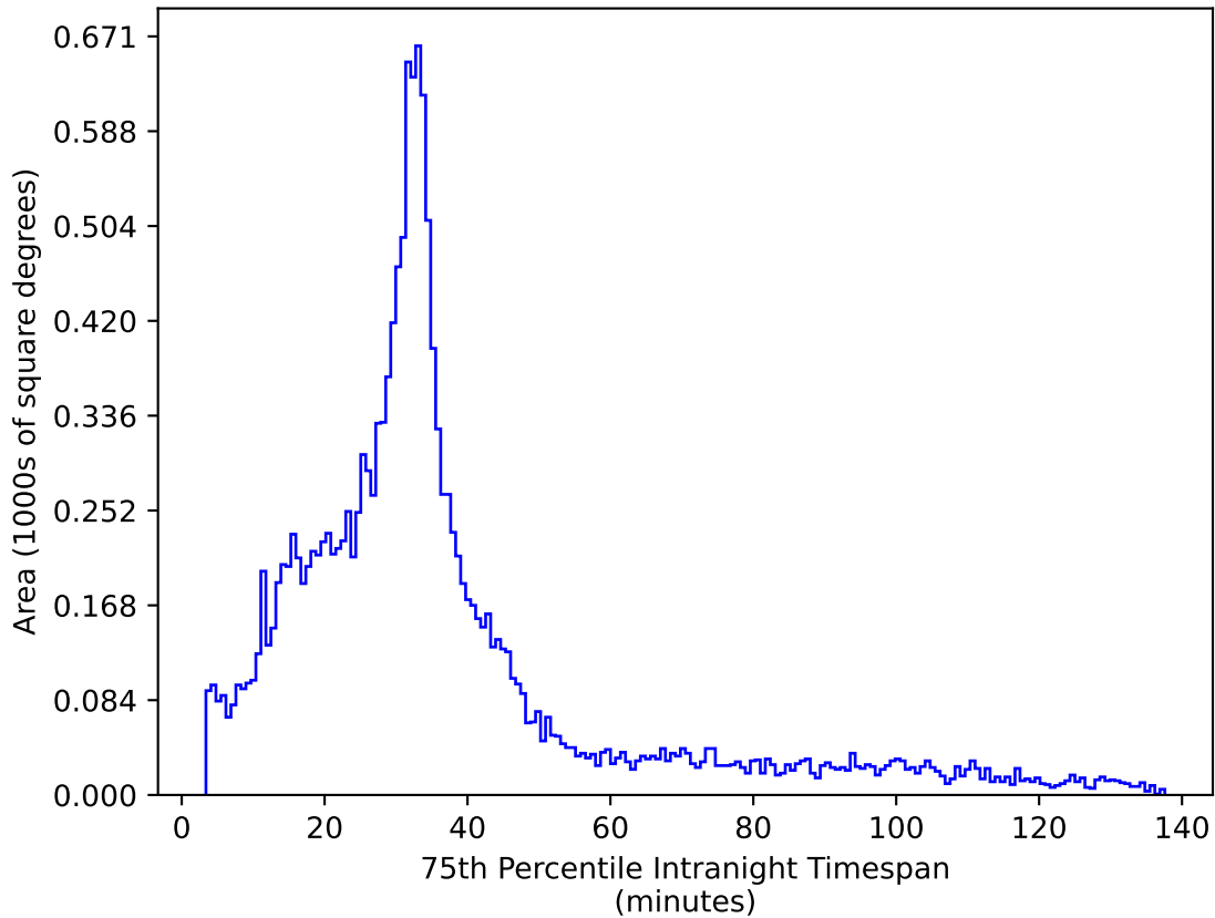
baseline_v2.0_10yrs WFD i band: 75th Percentile Intranight Timespan
