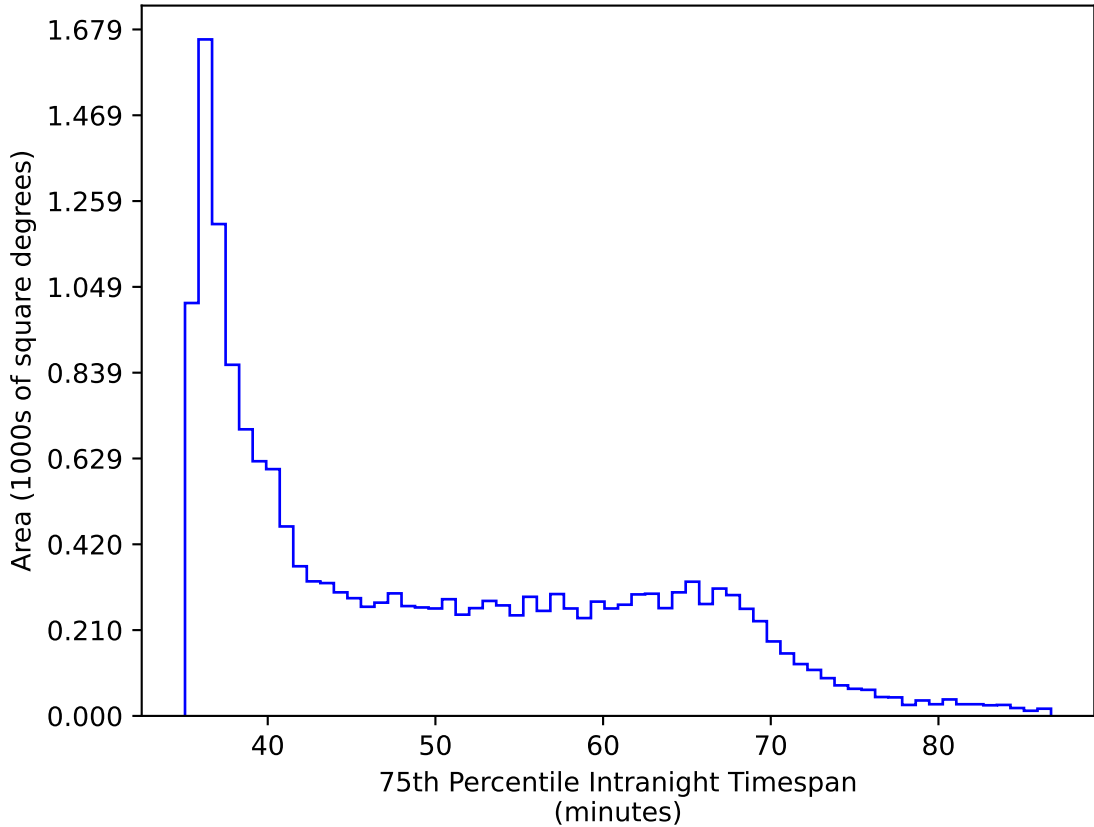
baseline_v2.0_10yrs WFD gr bands: 75th Percentile Intranight Timespan
