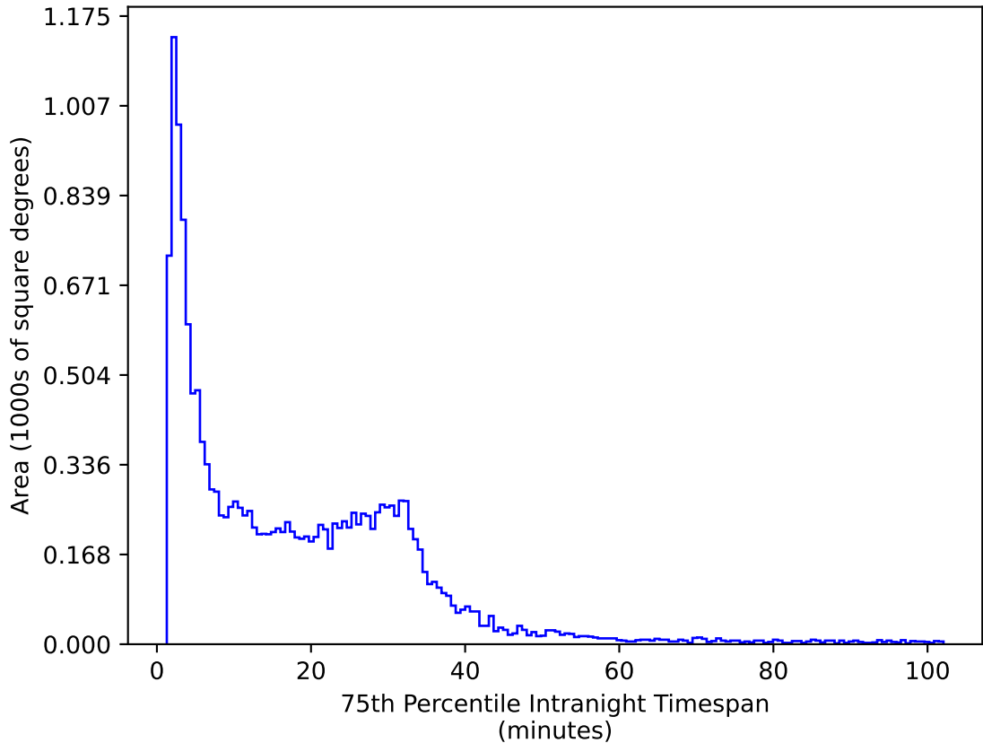
baseline_v2.0_10yrs WFD g band: 75th Percentile Intranight Timespan
