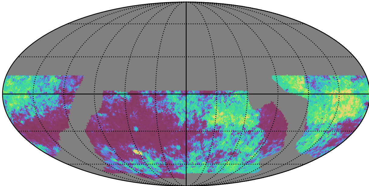
baseline_v2.0_10yrs WFD all bands: 75th Percentile Intranight Timespan
