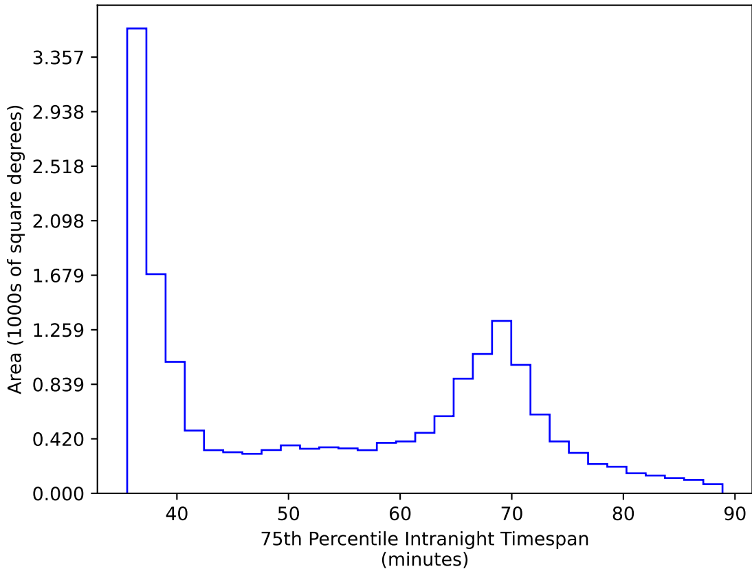
baseline_v2.0_10yrs WFD all bands: 75th Percentile Intranight Timespan
