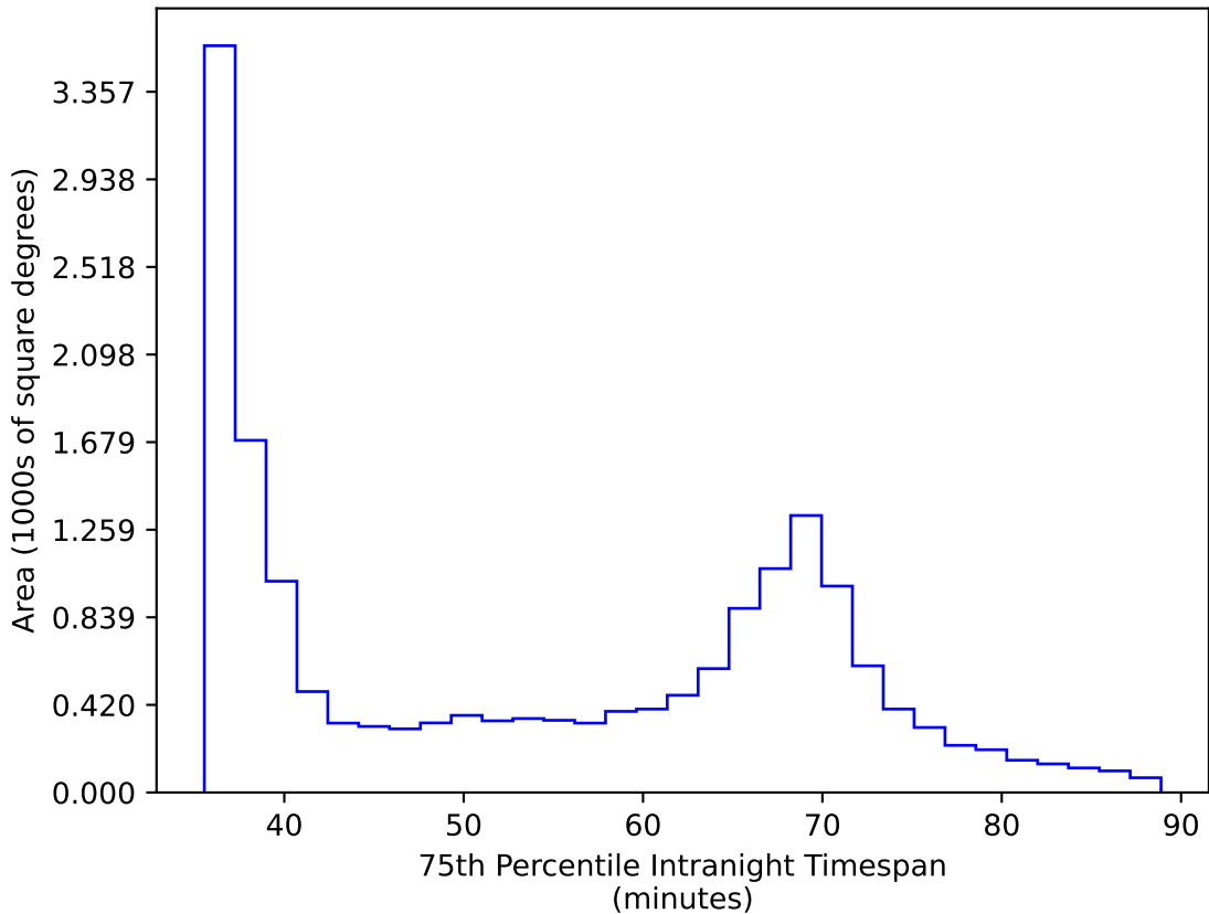
baseline_v2.0_10yrs WFD: 75th Percentile Intranight Timespan
