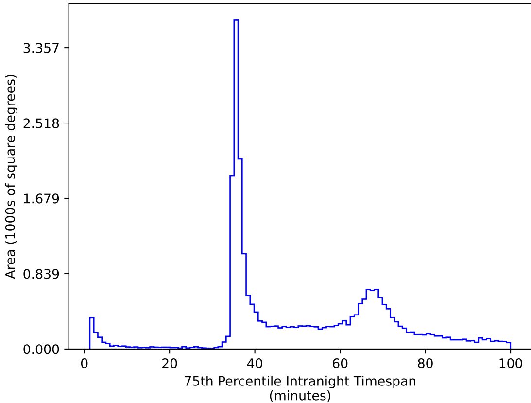
baseline_v2.0_10yrs All sky zy bands: 75th Percentile Intranight Timespan
