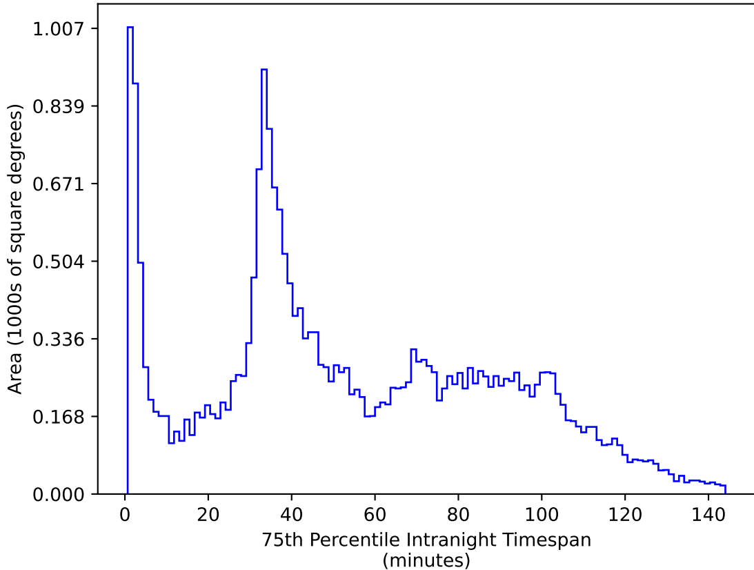
baseline_v2.0_10yrs All sky z band: 75th Percentile Intranight Timespan
