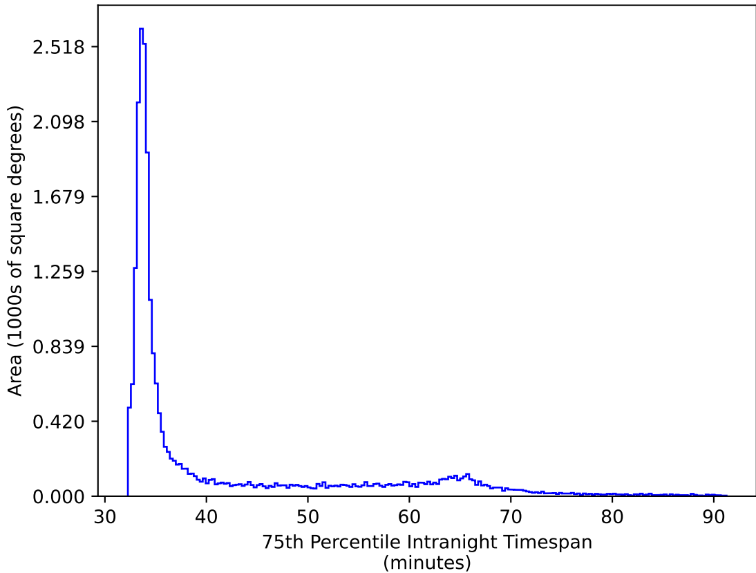
baseline_v2.0_10yrs All sky y band: 75th Percentile Intranight Timespan
