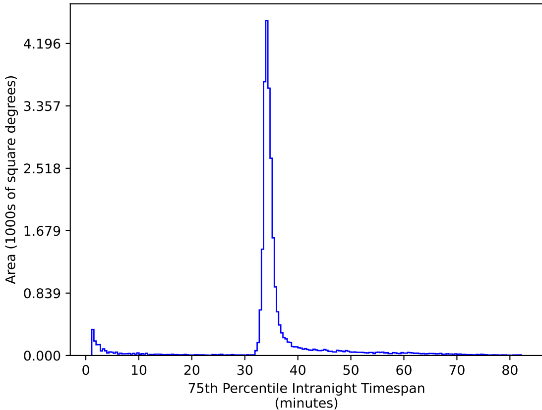
baseline_v2.0_10yrs All sky ug bands: 75th Percentile Intranight Timespan
