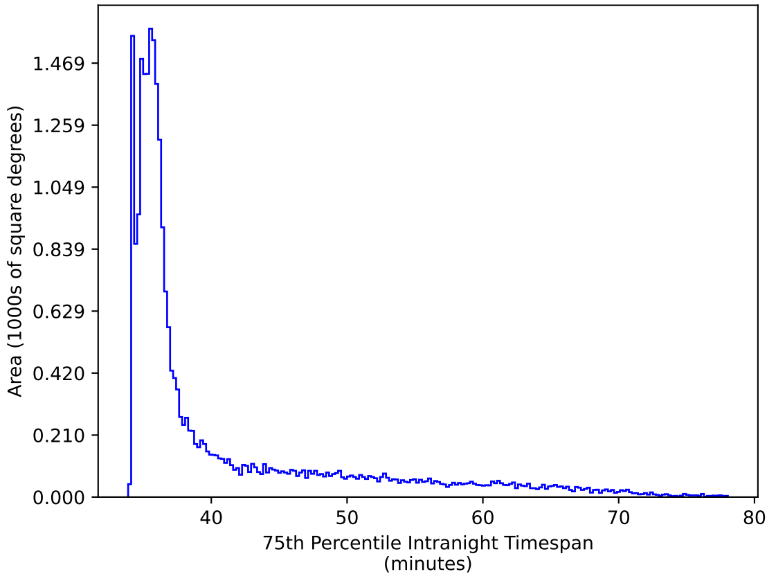
baseline_v2.0_10yrs All sky ri bands: 75th Percentile Intranight Timespan
