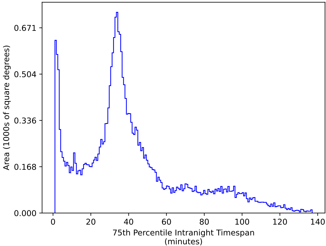
baseline_v2.0_10yrs All sky r band: 75th Percentile Intranight Timespan
