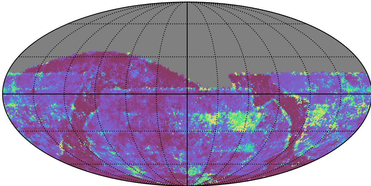
baseline_v2.0_10yrs All sky i band: 75th Percentile Intranight Timespan
