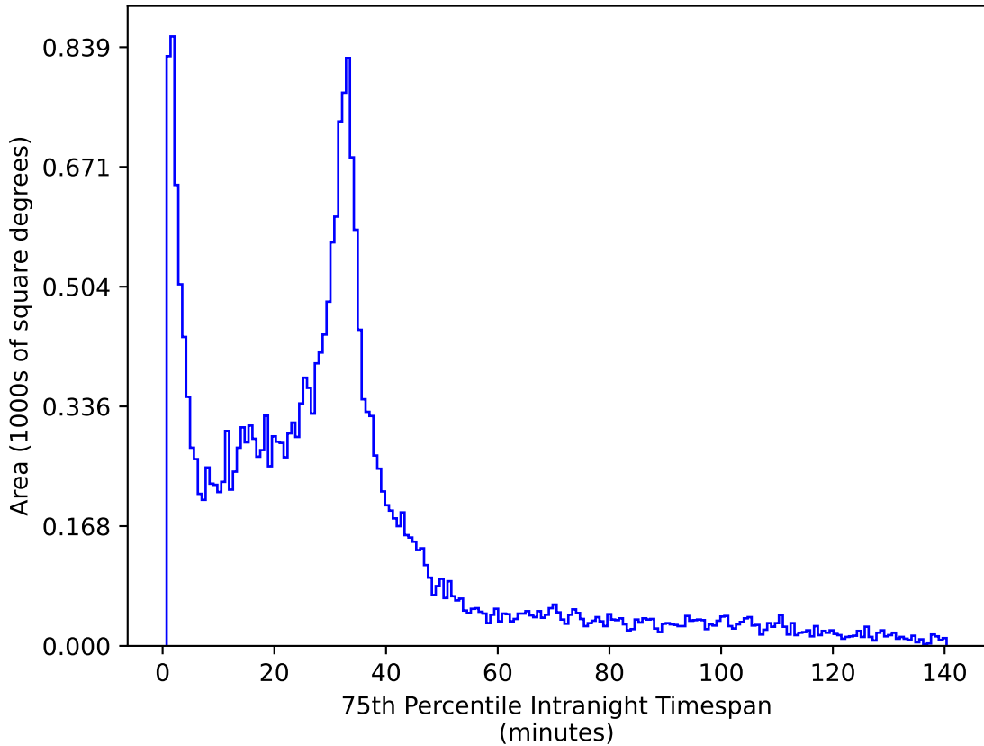
baseline_v2.0_10yrs All sky i band: 75th Percentile Intranight Timespan
