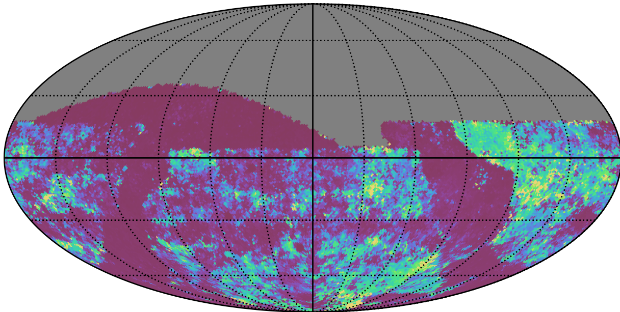
baseline_v2.0_10yrs All sky gr bands: 75th Percentile Intranight Timespan
