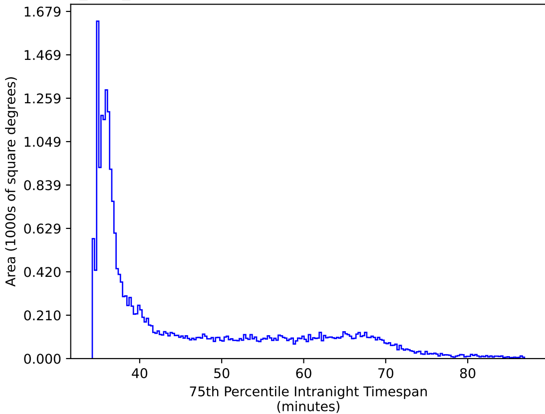
baseline_v2.0_10yrs All sky gr bands: 75th Percentile Intranight Timespan
