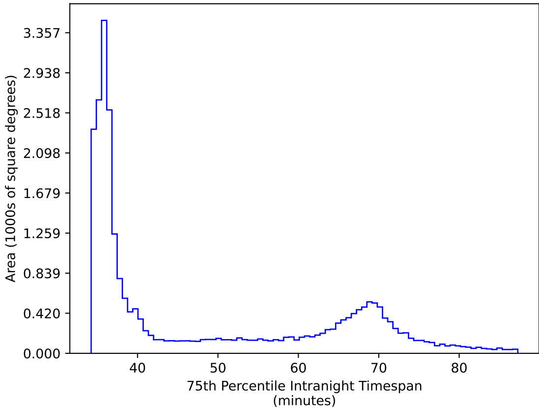
baseline_v2.0_10yrs All sky all bands: 75th Percentile Intranight Timespan
