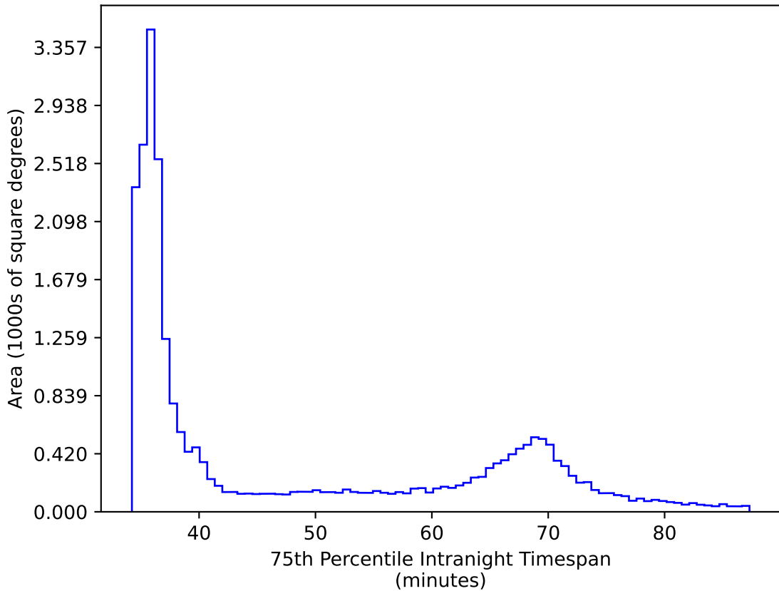
baseline_v2.0_10yrs All sky: 75th Percentile Intranight Timespan
