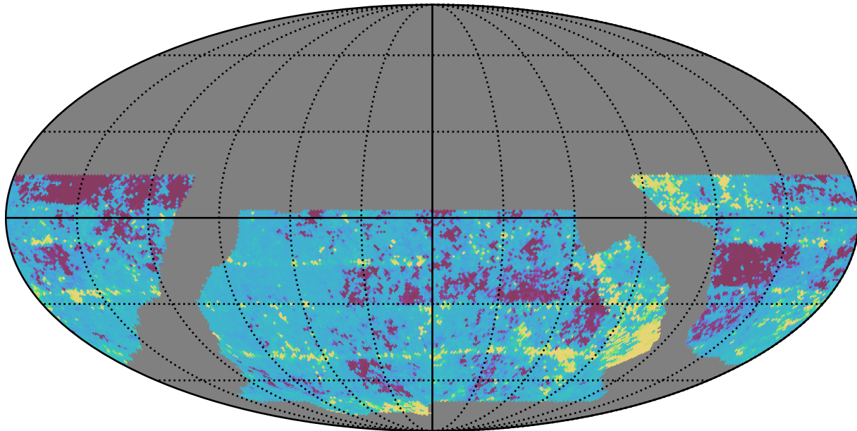
baseline_v2.0_10yrs WFD z band: 20thPercentile Inter-Night Gap
