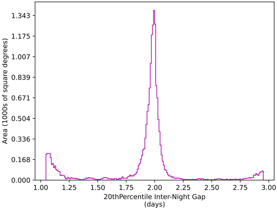
baseline_v2.0_10yrs WFD z band: 20thPercentile Inter-Night Gap
