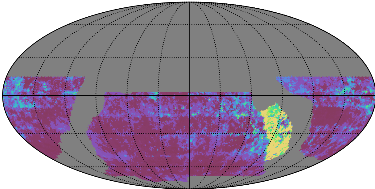
baseline_v2.0_10yrs WFD y band: 20thPercentile Inter-Night Gap
