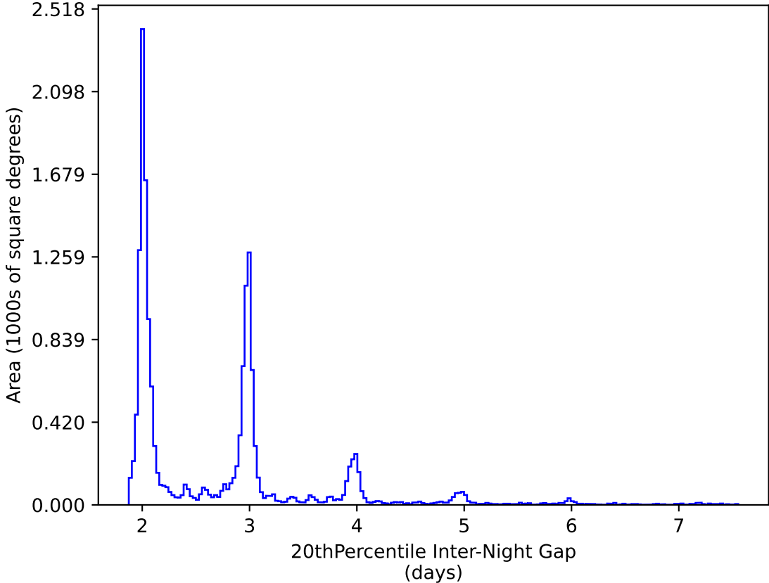
baseline_v2.0_10yrs WFD y band: 20thPercentile Inter-Night Gap
