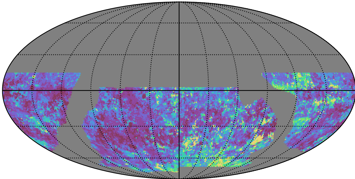
baseline_v2.0_10yrs WFD u band: 20thPercentile Inter-Night Gap
