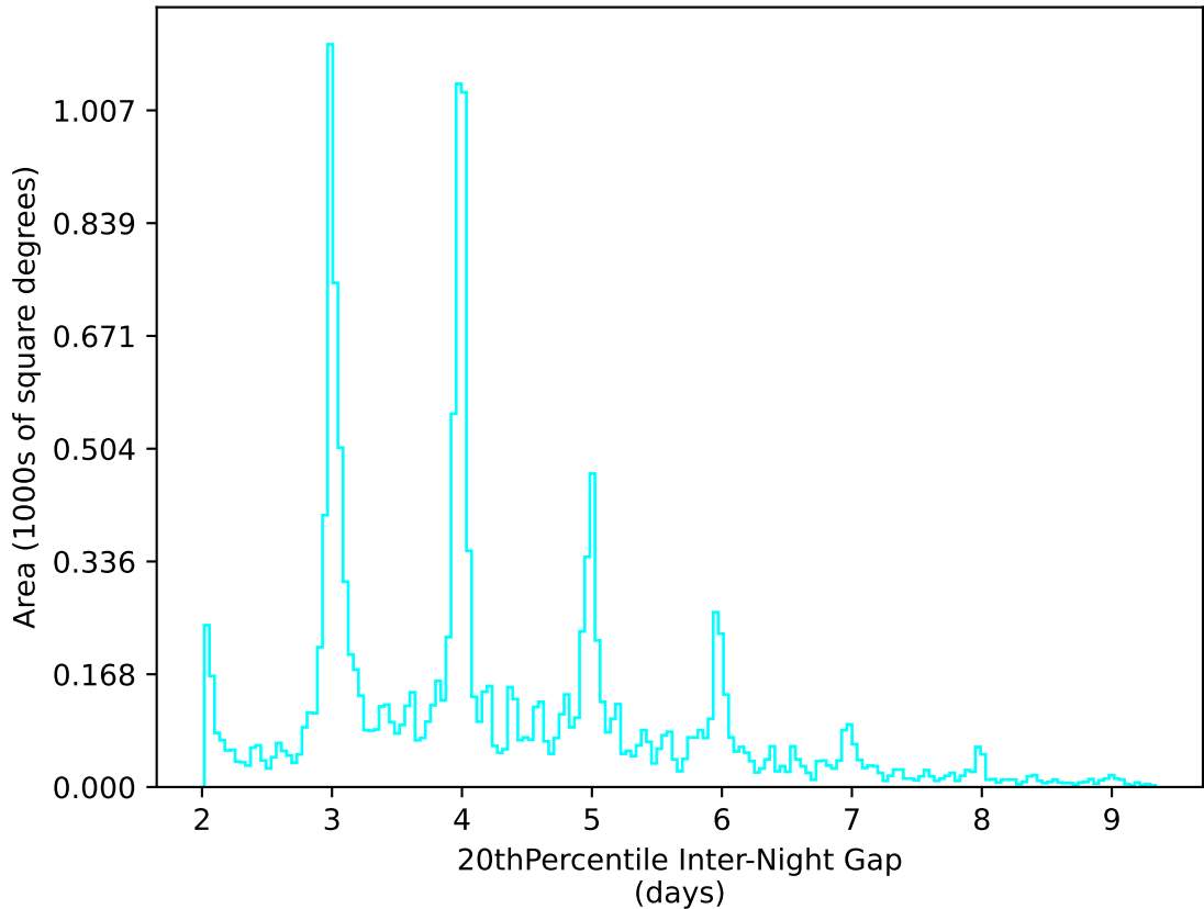
baseline_v2.0_10yrs WFD u band: 20thPercentile Inter-Night Gap
