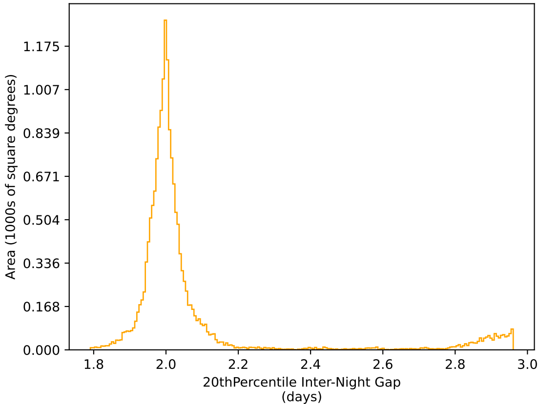
baseline_v2.0_10yrs WFD r band: 20thPercentile Inter-Night Gap
