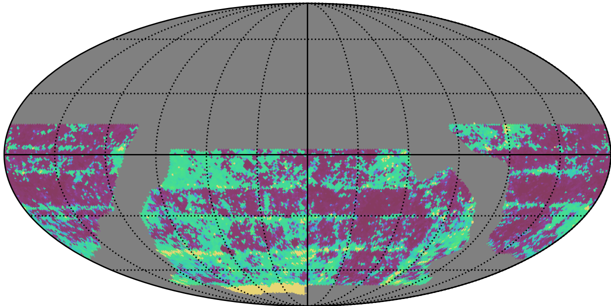
baseline_v2.0_10yrs WFD i band: 20thPercentile Inter-Night Gap
