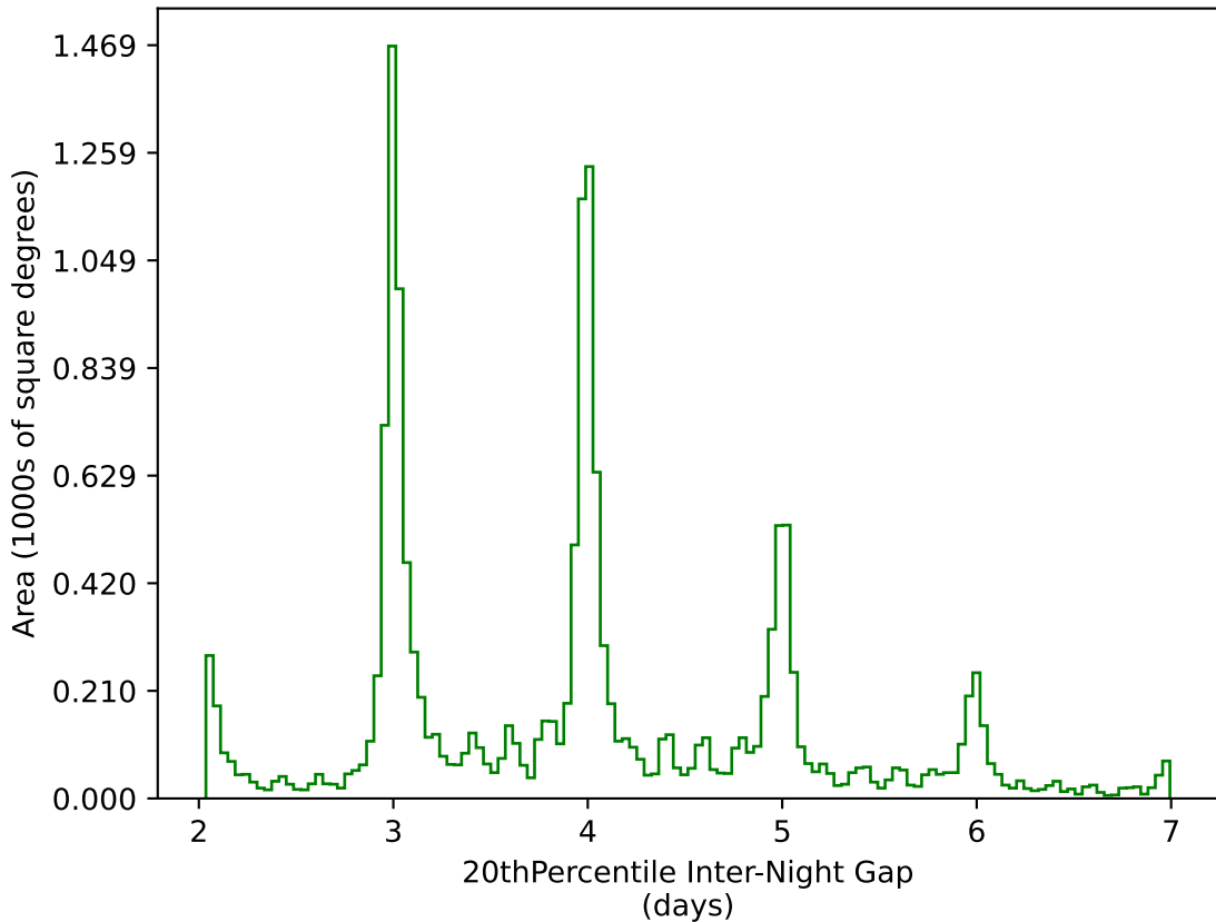
baseline_v2.0_10yrs WFD g band: 20thPercentile Inter-Night Gap
