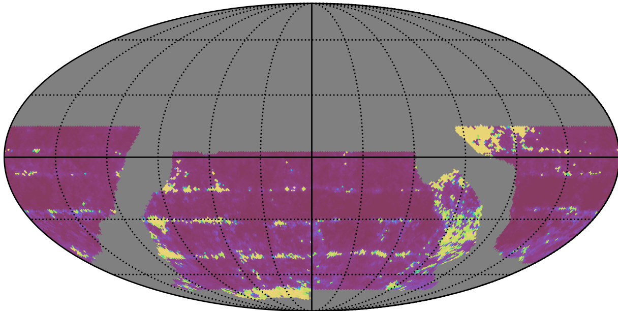
baseline_v2.0_10yrs WFD all bands: 20thPercentile Inter-Night Gap
