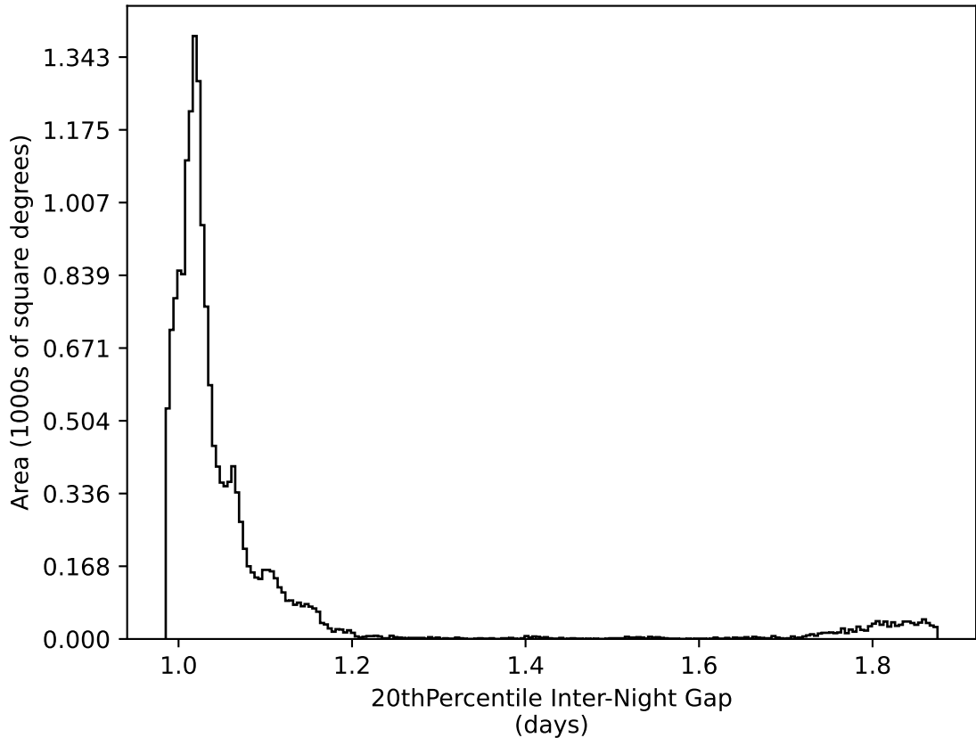
baseline_v2.0_10yrs WFD all bands: 20thPercentile Inter-Night Gap
