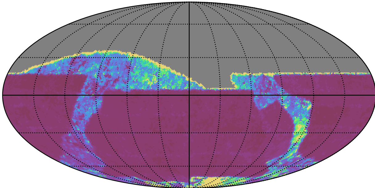
baseline_v2.0_10yrs All sky z band: 20thPercentile Inter-Night Gap
