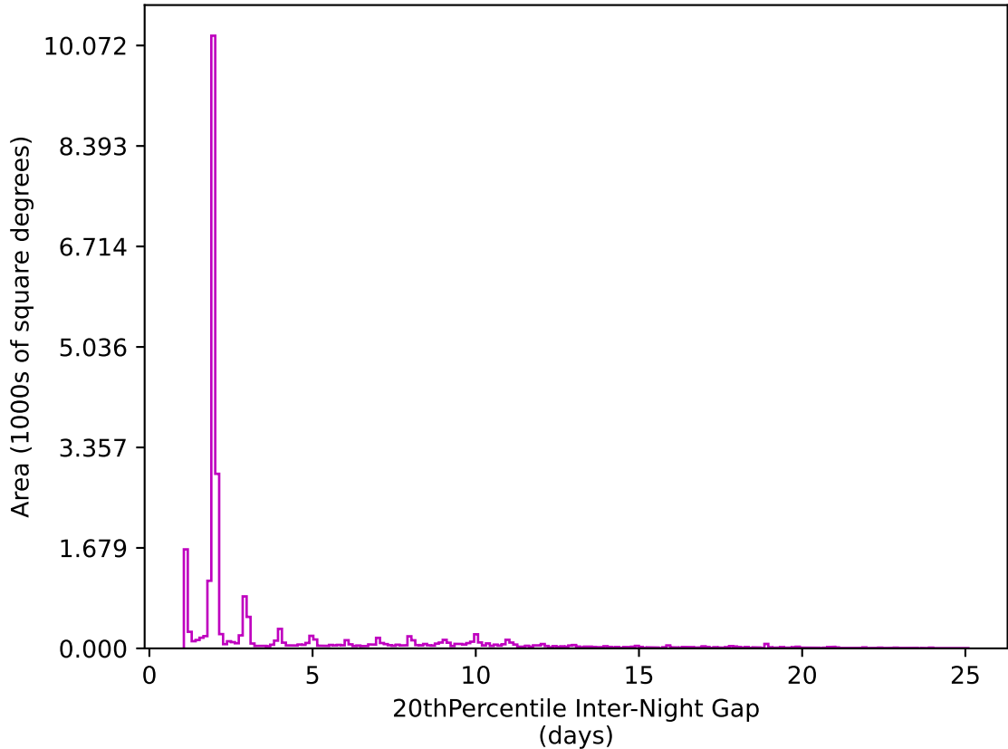
baseline_v2.0_10yrs All sky z band: 20thPercentile Inter-Night Gap
