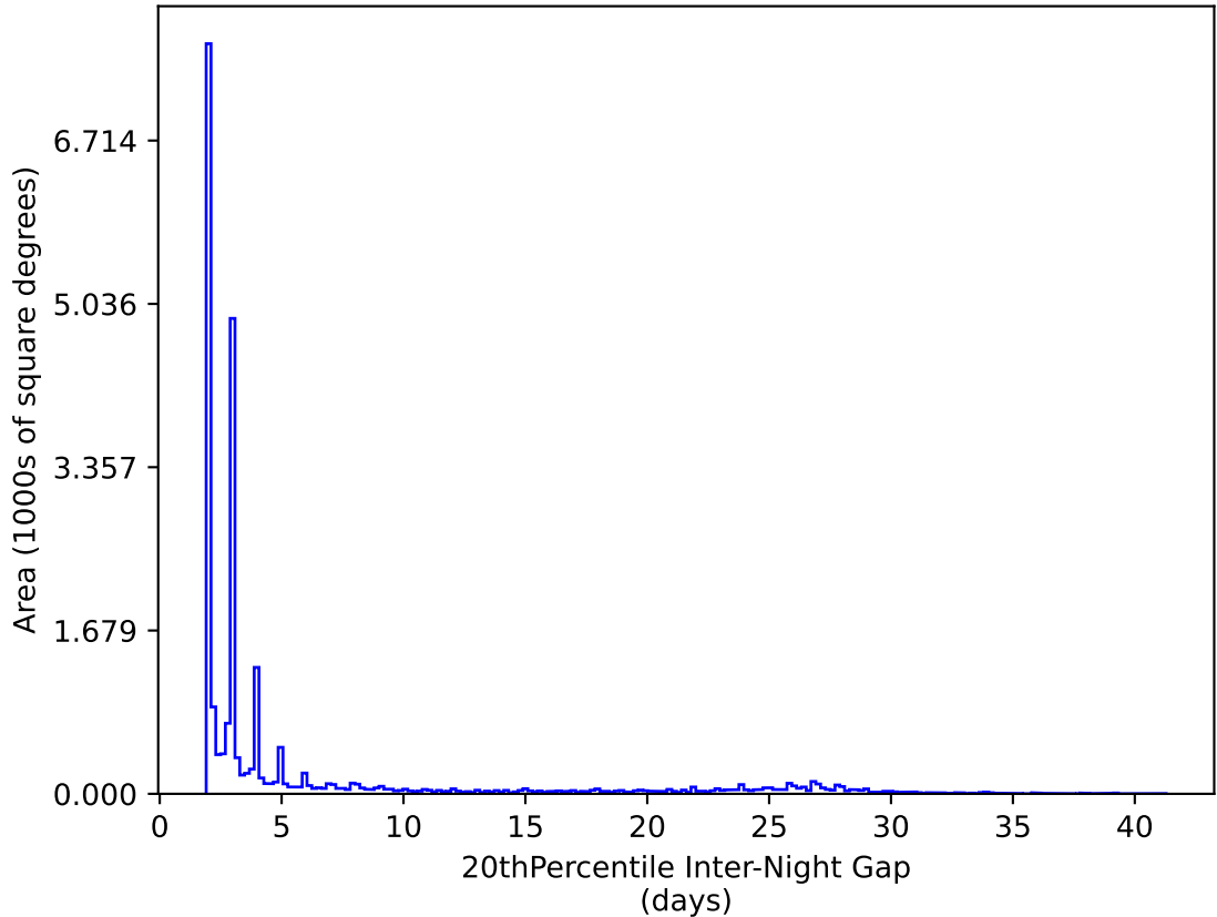
baseline_v2.0_10yrs All sky y band: 20thPercentile Inter-Night Gap
