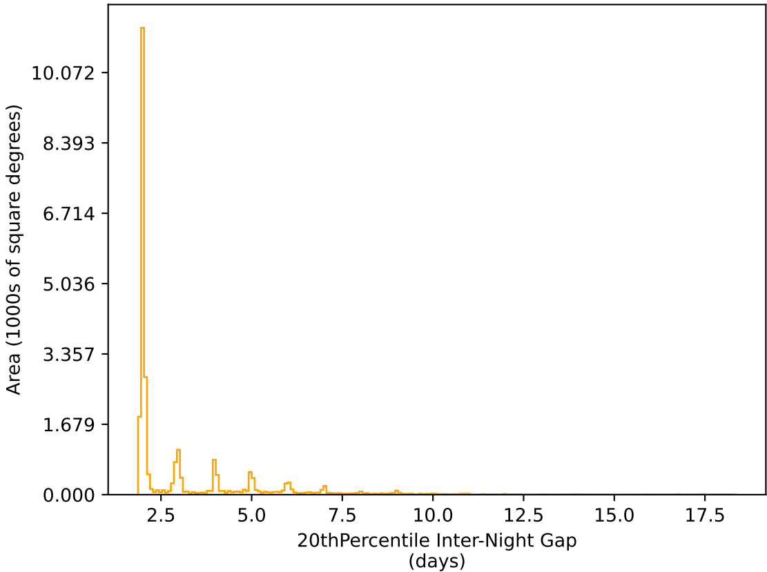
baseline_v2.0_10yrs All sky r band: 20thPercentile Inter-Night Gap
