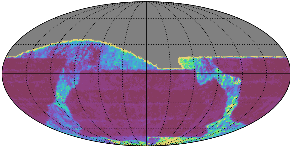
baseline_v2.0_10yrs All sky i band: 20thPercentile Inter-Night Gap
