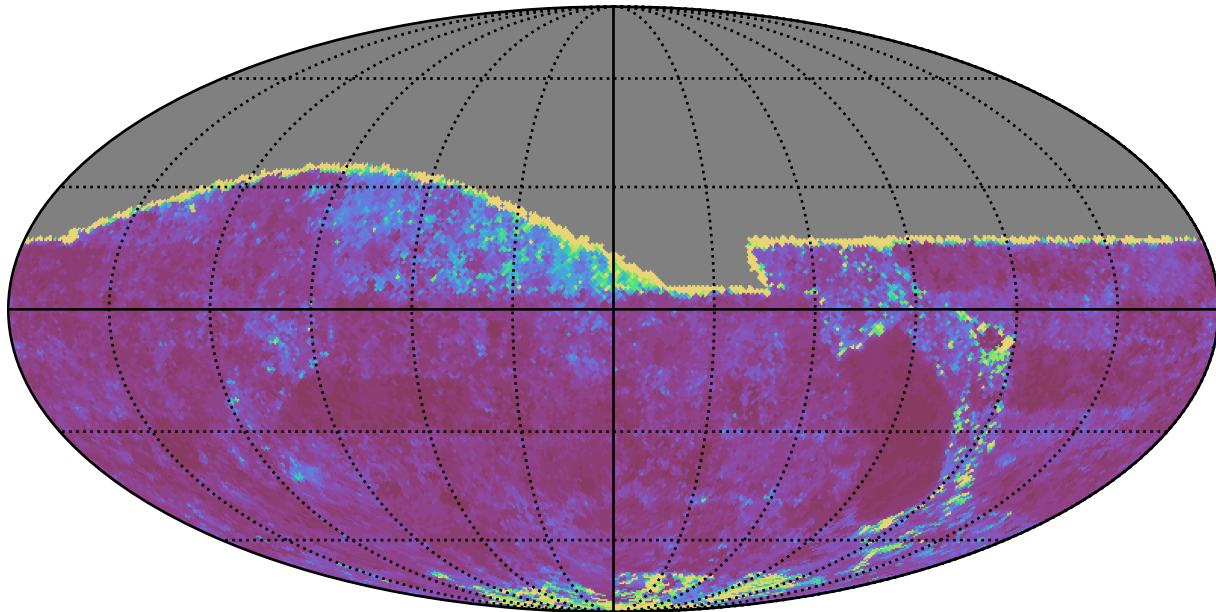
baseline_v2.0_10yrs All sky g band: 20thPercentile Inter-Night Gap
