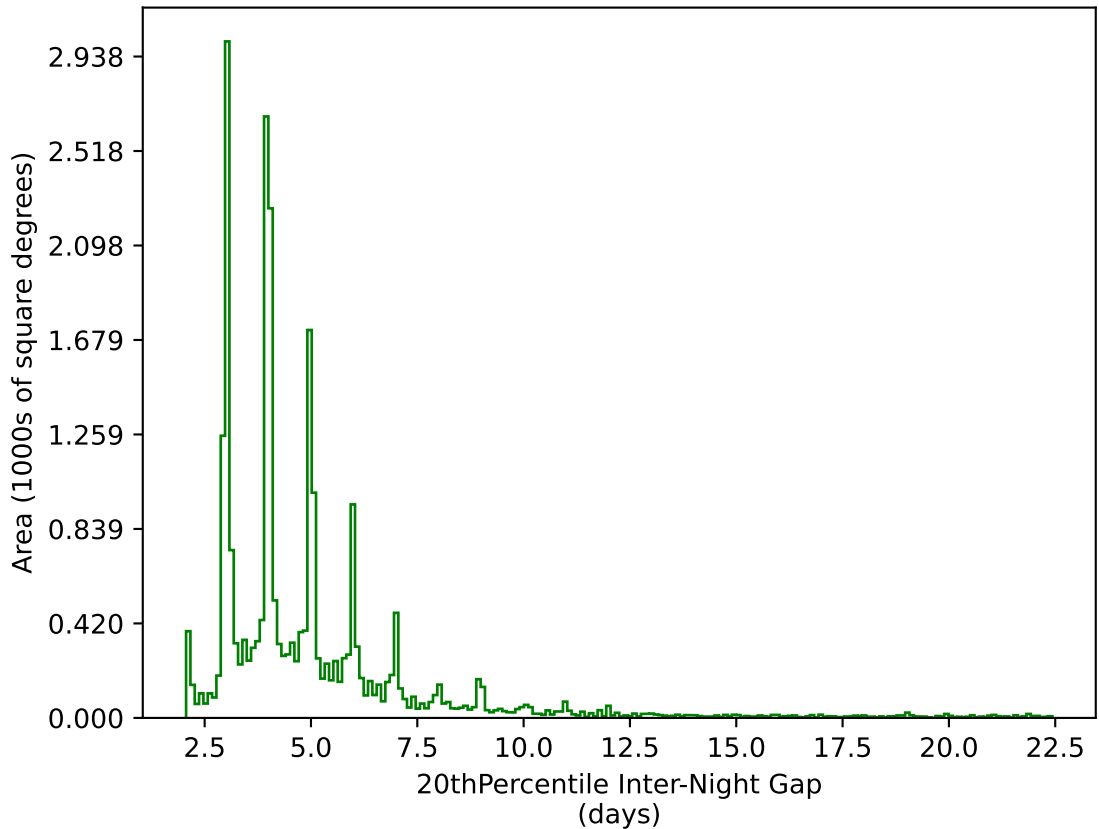
baseline_v2.0_10yrs All sky g band: 20thPercentile Inter-Night Gap
