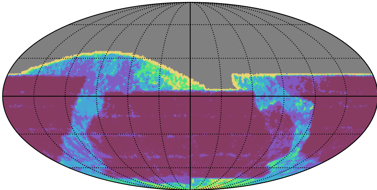
baseline_v2.0_10yrs All sky all bands: 20thPercentile Inter-Night Gap
